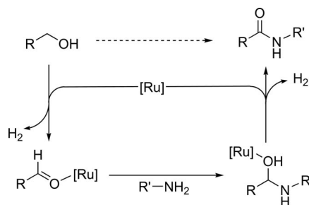
Scheme 1. Ru-catalyzed amide formation from alcohols and amines.
