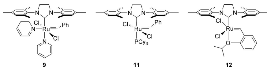
Figure 2. NHC-based Ru olefin-metathesis catalysts.
