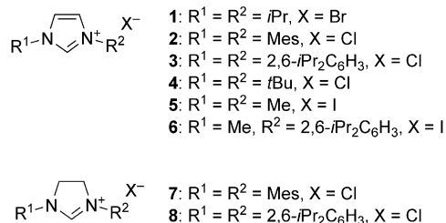
Figure 1. NHC precursors.
